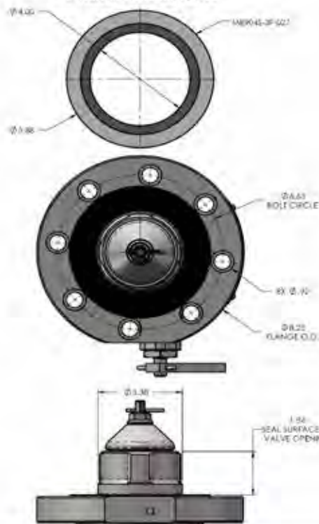
ME990-3DFM SERIES 3" FLANGED INTERNAL VALVES
