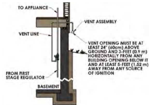
Figure 4: Basement Installation
